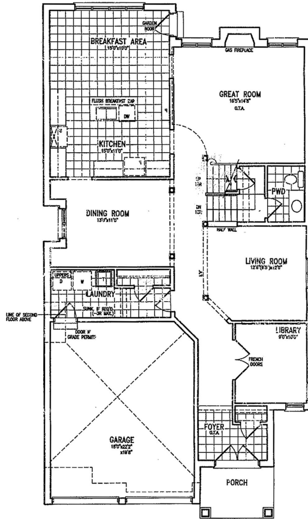
GROUND FLOOR PLAN 'B' (4 BEDROOM)
