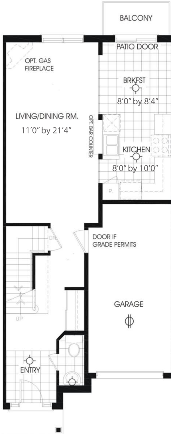
GROUND FLOOR PLAN 2 STOREY
