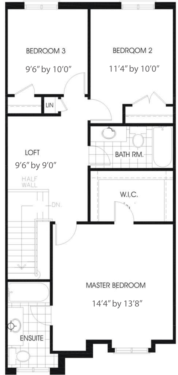
SECOND FLOOR PLAN - OPT. 3 BDRM 2 STOREY
